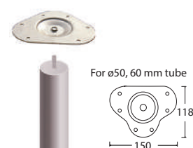
71557 Steel plate
